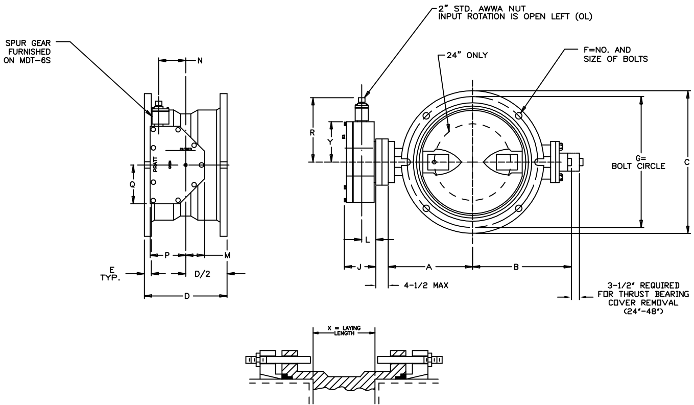
INSTALLATION DIAGRAM NOTE: BOLTS, NUTS, GLANDS AND GASKETS FURNISHED BY OTHERS.
