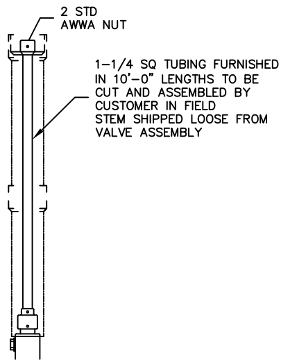
OPTIONAL EXTENSION STEM ARRANGEMENT
